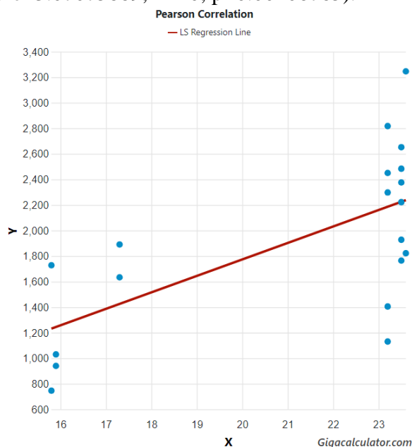
Fig. 1. Correlation between mean ocean water temperature and curved surface area in Centrobolus Cook, 1897.
