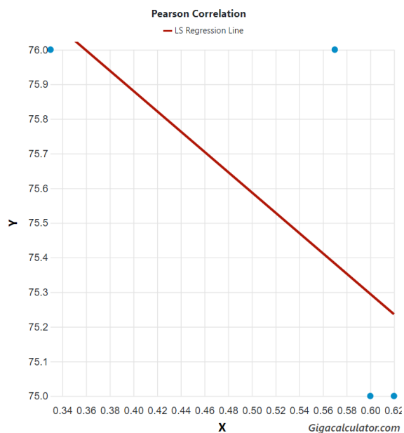
Figure 1. Correlation between sex ratio and humidity in two species of Centrobolus .
