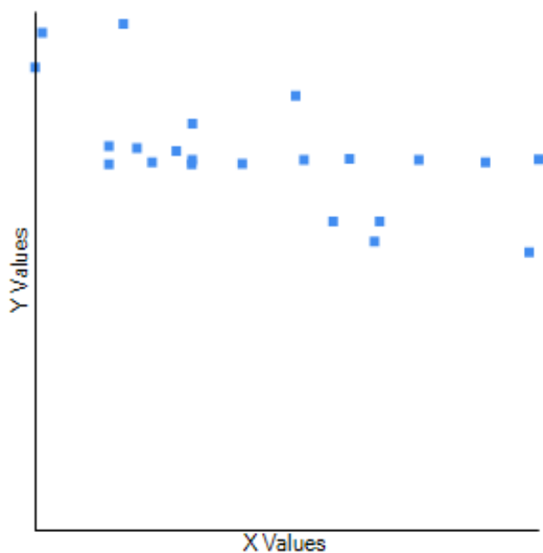
Fig. 2. Correlation between hours of sunshine throughout the year (h) and curved surface area in males in Centrobolus Cook, 1897.
