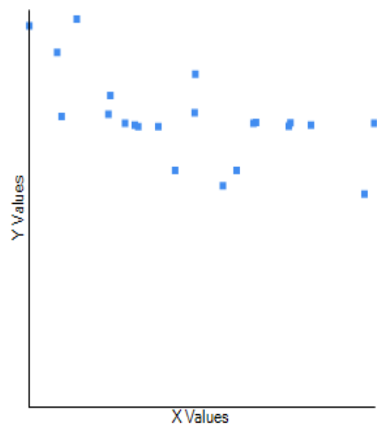
Fig. 1. Correlation between hours of sunshine throughout the year (h) and curved surface area in females in Centrobolus Cook , 1897.
