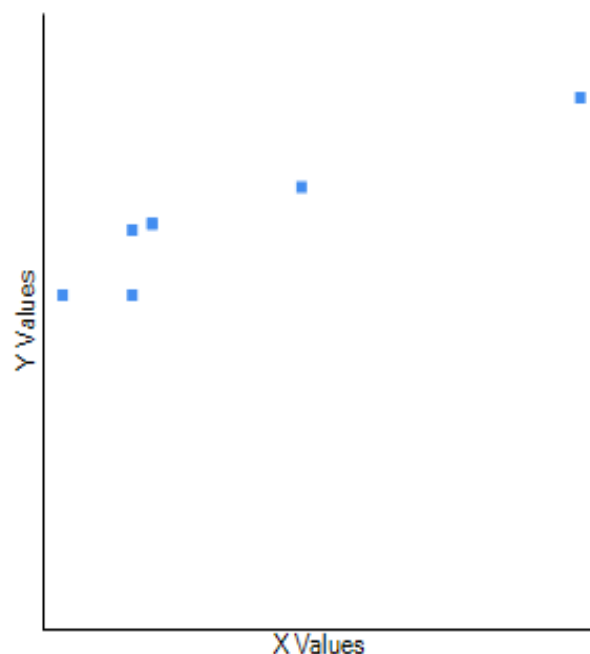
Fig. 1 A correlation between the mean annual temperature with the lowest average temperature across the distribution of pill millipedes Sphaerotherium .
