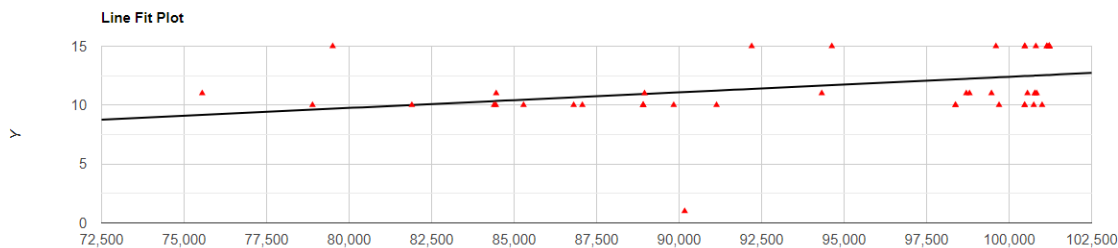
Fig. 1. Correlation between longitudinal species richness (Y) and air pressure (X) across the range of Sphaerotheriidae Brandt, 1833.
