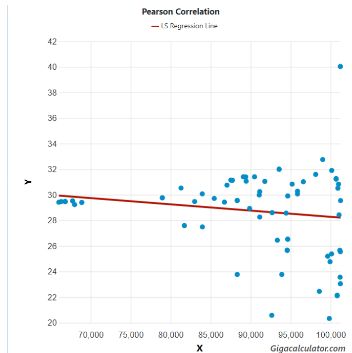
Fig. 1. Correlation between longitude (Y) and air pressure (X) across the range of Gnomeskelus Attems, 1926.
