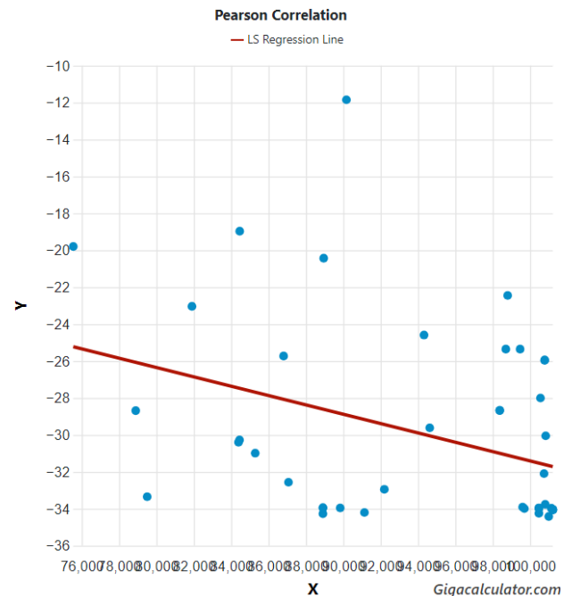
Fig. 1. Correlation between latitude (Y) and air pressure (X) across the range of Sphaerotherium Brandt, 1833.
