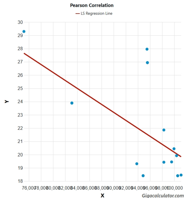
Fig. 1. Correlation between longitude (Y) and air pressure (X) across the range of Julomorphidae Verhoeff, 1924.
