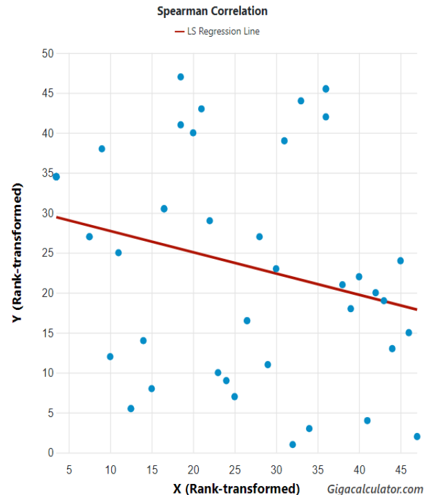
Fig. 1. Correlation between longitude (Y) and air pressure (X) across therange of Sphaerotheriidae Brandt, 1833.
