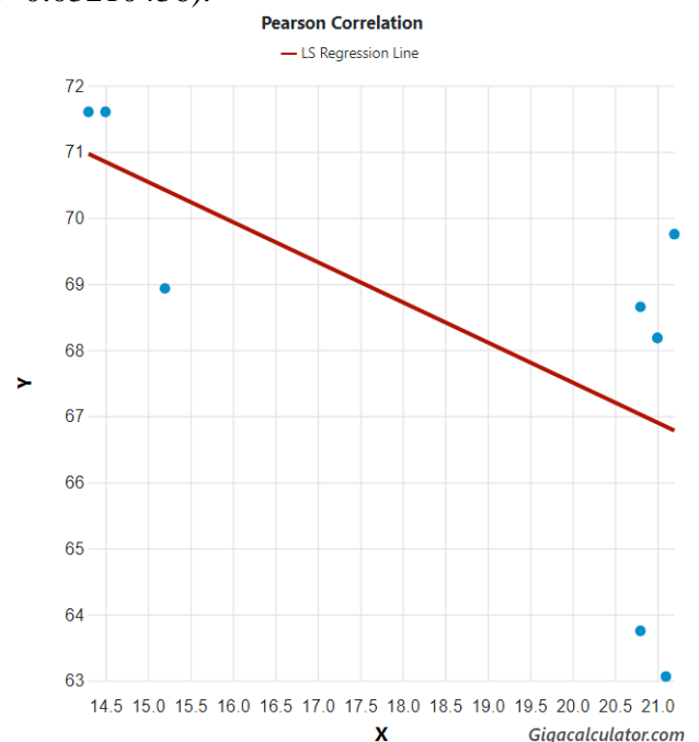
Fig. 1. Correlation between minimum ocean water temperature (x) and highest relative humidity (y) across the range of Centrobolus Cook, 1897.
