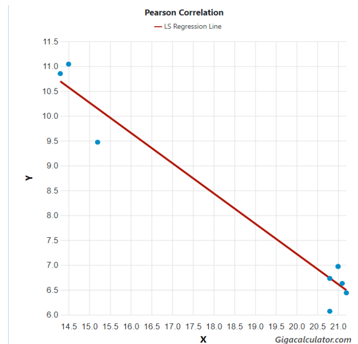
Fig. 1. Correlation between minimum ocean water temperature (x) and lowest number of daily hours of sunshine (y) across the range of Centrobolus Cook, 1897.
