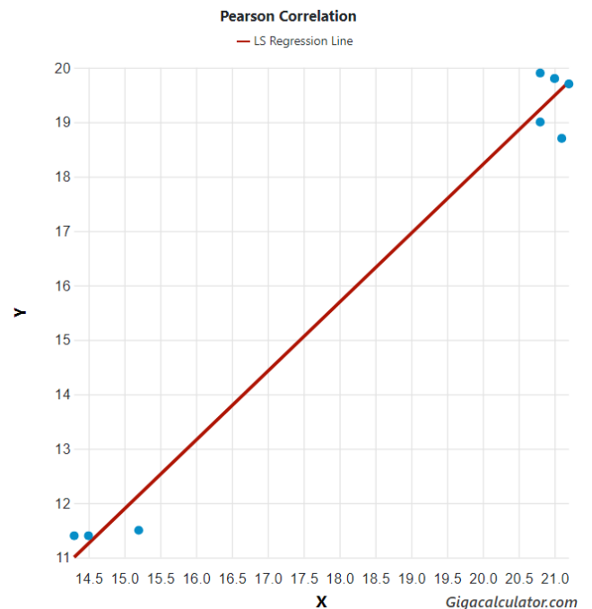
Fig. 1. Correlation between minimum ocean water temperature (x) and minimum temperature (y) across the range of Centrobolus Cook, 1897.
