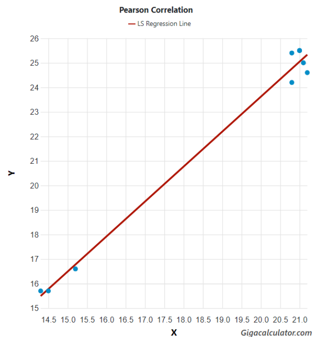
Fig. 1. Correlation between minimum ocean water temperature (x) and maximum temperature (y) across the range of Centrobolus Cook, 1897.
