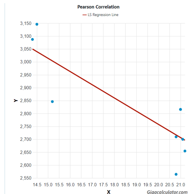
Fig. 1. Correlation between minimum ocean water temperature (x) and the hours of sunshine throughout the year (y) across the range of Centrobolus Cook, 1897.
