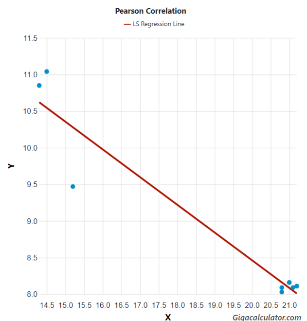
Fig. 1. Correlation between minimum ocean water temperature (x) and month with the highest duration of sunshine (y) across the range of Centrobolus Cook, 1897.
