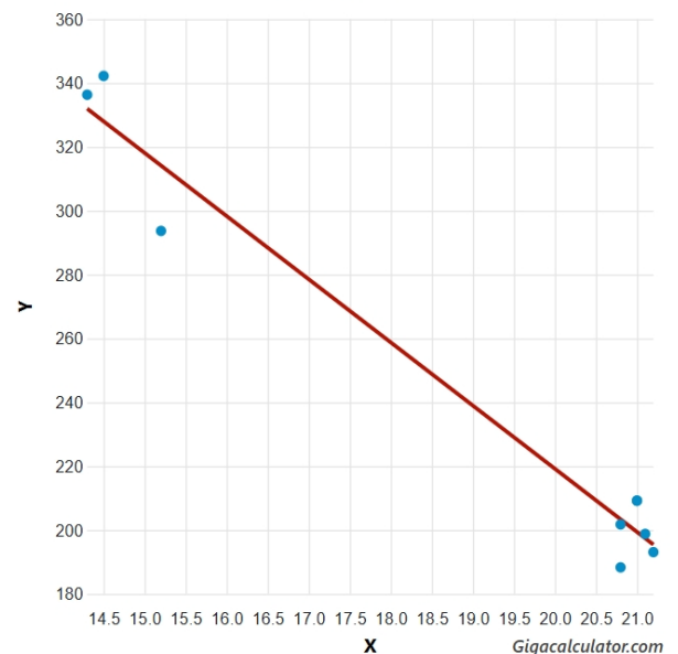
Fig. 1. Correlation between minimum ocean water temperature (x) and lowest duration of sunshine (y) across the range of Centrobolus Cook, 1897.
