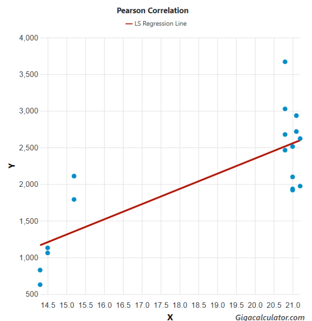
Fig. 1. Correlation between minimum ocean water temperature (x) and surface area (y) across the range of Centrobolus Cook, 1897.
