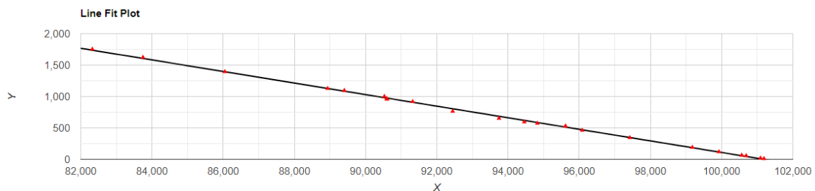
Figure 1. Correlation showing air pressure was correlated with altitude in southern African Harpagophoridae.
