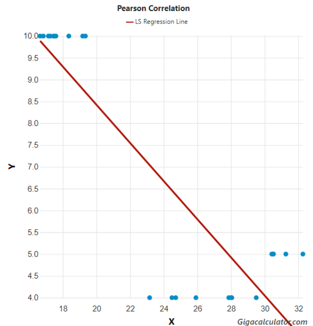
Figure 1. Correlation between species richness and longitude in southern African Harpagophoridae Attems, 1909.
