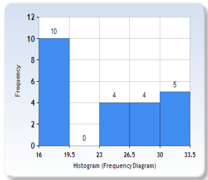
Figure 2. Longitudinal species richness in southern African Harpagophoridae Attems, 1909.
