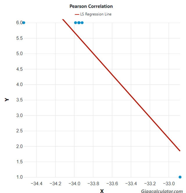
Figure 2. Correlation between latitude and species richness in introduced species of southern African Diplopoda.
