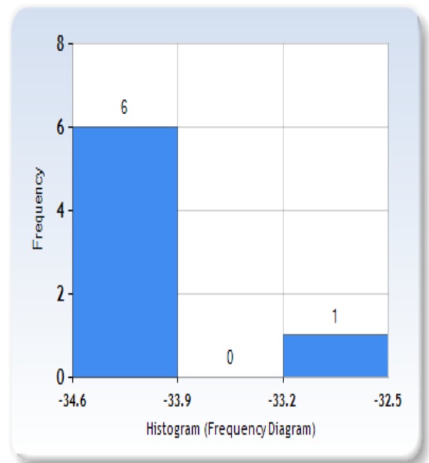
Figure 1. Latitudinal species distribution in introduced species of southern African Diplopoda.
