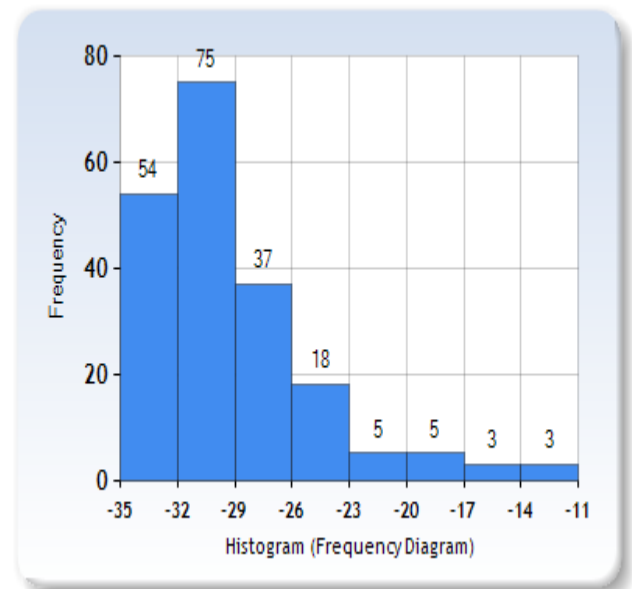
Figure 1. Latitudinal species richness in southern African Juliformia Attems, 1926.
