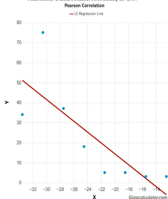
Figure 2. Latitudinal species richness in southern African Juliformia Attems, 1926 as latitude (x) versus species richness (y).
