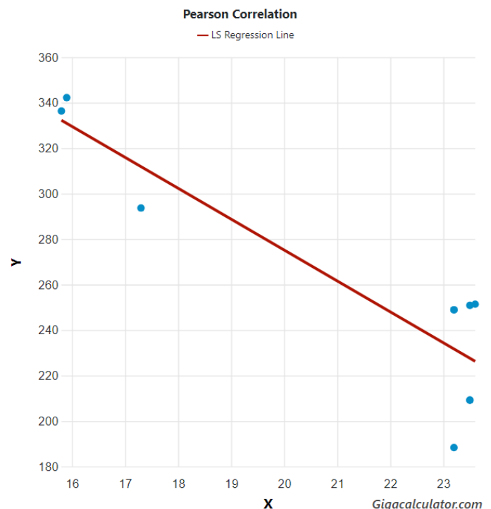
Fig. 1. Correlation between highest number of daily hours of sunshine in a month (y) and mean ocean water temperature (x) across the range of Centrobolus Cook , 1897.
