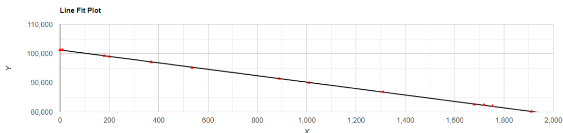
Figure 1. Correlation between air pressure and elevation in southern African Patinatius Attems, 1928.
