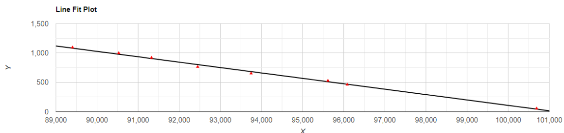
Figure 1. Altitude correlated with air pressure in southern African Harpagophora Attems, 1909.
