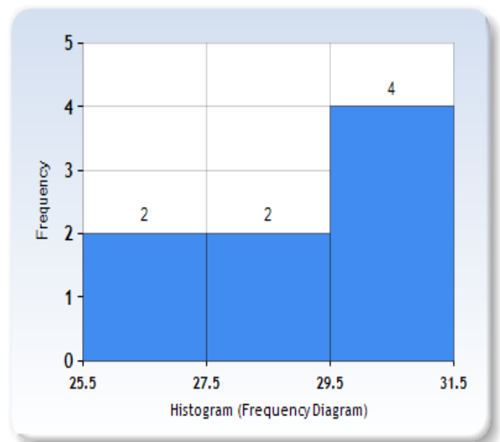
Figure 2. Longitudinal species richness in southern African Camaricoproctus Attems, 1926.
