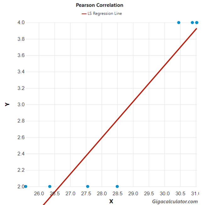
Figure 1. Longitude versus species richness in southern African Camaricoproctus Attems, 1926.
