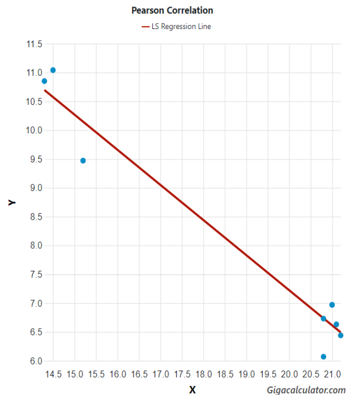
Fig. 1. Correlation between lowest number of daily hours of sunshine in a month (Y) and minimum ocean water temperature (X) across the range of Centrobolus Cook, 1897.
