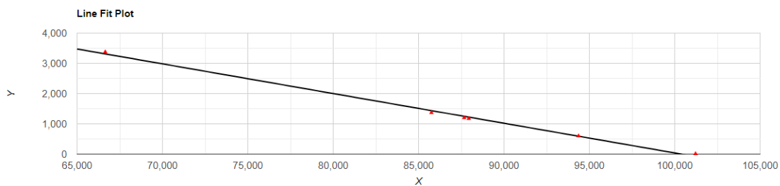
Figure 1. Air pressure and altitude correlation in southern African Phygoxerotes .
