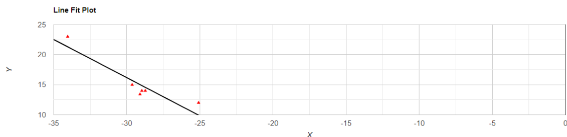
Figure 1. Temperature and latitude correlation in southern African Phygoxerotes .
