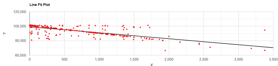
Figure 1. Altitude correlated to air pressure in southern African Juliformia Attems, 1926.
