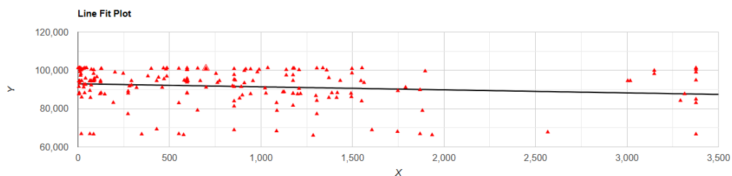
Figure 1. Air pressure correlated to altitude in southern African Polydesmida Leach, 1815.
