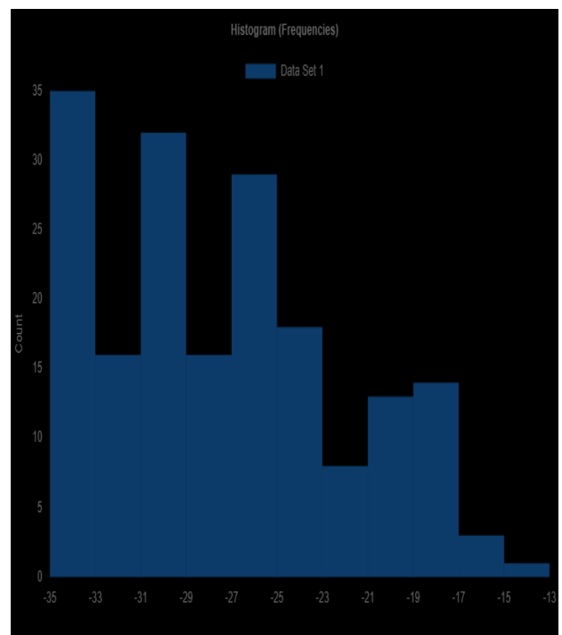
Figure 2. Latitudinal species richness in southern African Polydesmida Leach, 1815.
