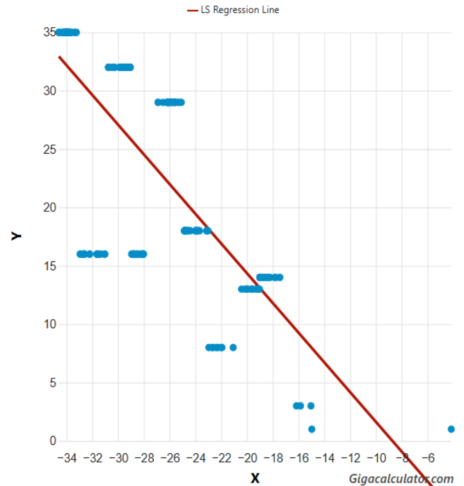
Figure 1. Species richness correlated to latitude in southern African Polydesmida Leach, 1815.
