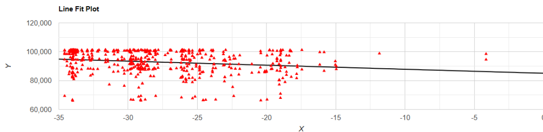
Figure 1. Air pressure correlated to latitude in southern African Diplopoda Blainville in Gervais, 1844.
