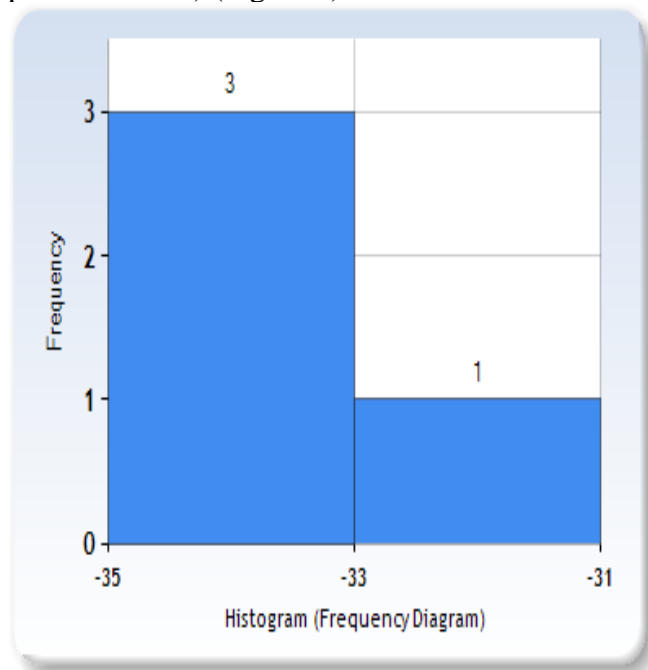
Figure 1. Latitudinal species richness in Antiphonus Attems, 1901.
