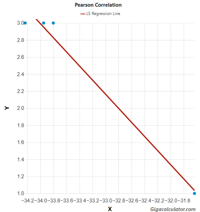
Figure 2. Latitude correlated with species richness in Antiphonus Attems, 1901.
