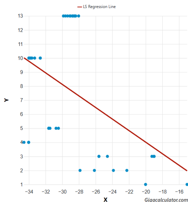
Figure 1. Latitude correlated to species richness in southern African Pachybolidae Cook, 1897.
