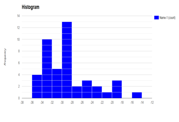
Figure 2. Latitudinal species richness in southern African Pachybolidae Cook, 1897.
