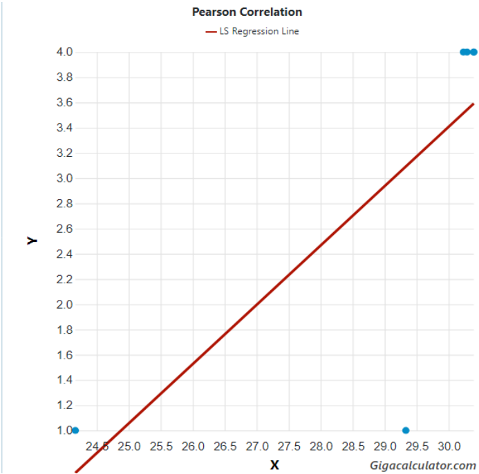
Figure 1. Longitude correlated with species richness in southern African Rhopaloskelus Attems, 1940.
