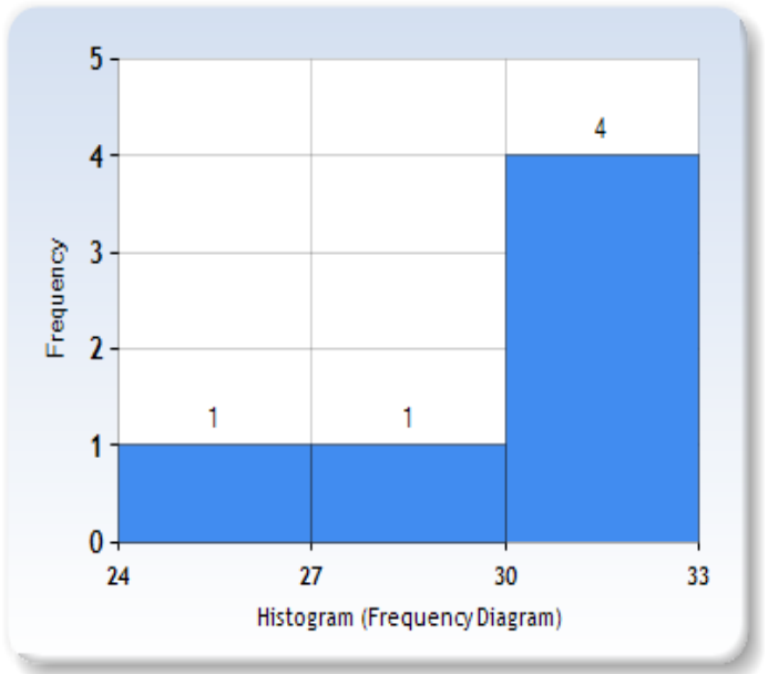
Figure 2. Longitudinal species richness in southern African Rhopaloskelus Attems, 1940.
