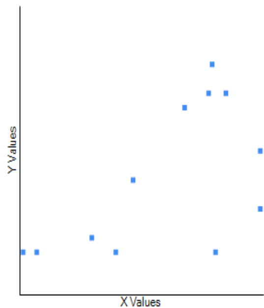
Fig. 8. Correlation between maximum temperature and rainy days in Bandula.
