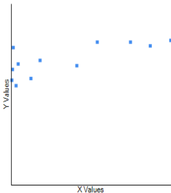
Fig. 9. Correlation between precipitation and humidity in Bandula.
