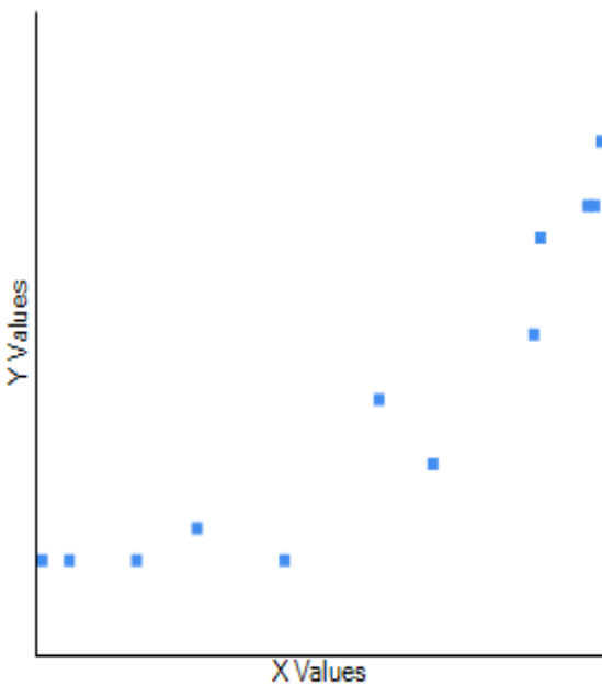
Fig. 7. Correlation between minimum temperature and rainy days in Bandula.
