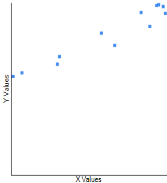
Fig. 1. Correlation between average temperature and minimum temperature in Bandula.
