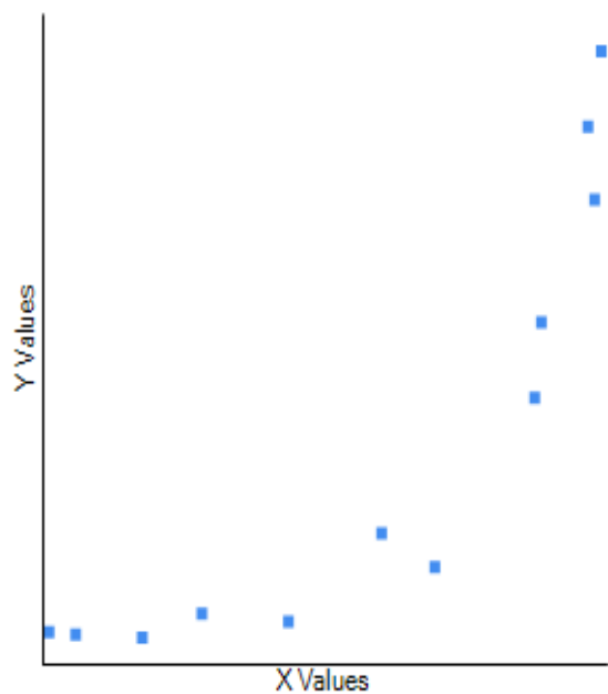
Fig. 6. Correlation between minimum temperature and precipitation in Bandula.
