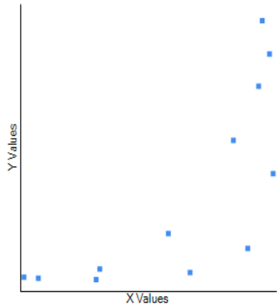
Fig. 3. Correlation between average temperature and precipitation in Bandula.
