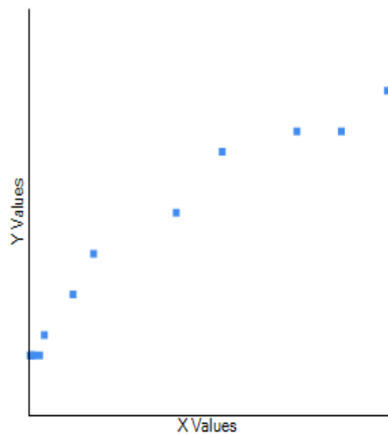
Fig. 10. Correlation between precipitation and rainy days in Bandula.
