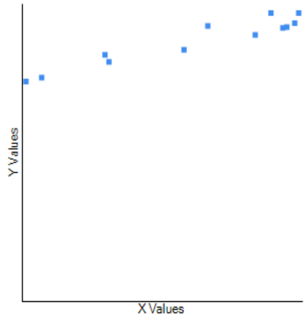
Fig. 2. Correlation between average and maximum temperature in Bandula.
