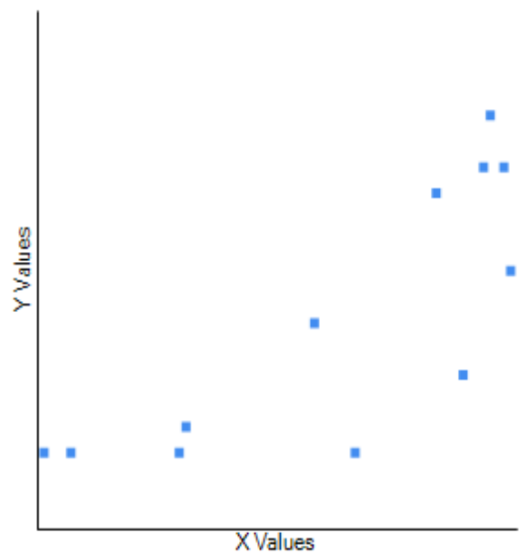
Fig. 4. Correlation between average temperature and rainy days in Bandula.
