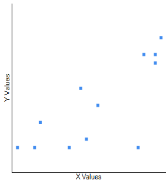
Fig. 11. Correlation between humidity and rainy days in Bandula.
