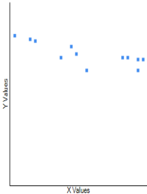
Fig. 12. Correlation between humidity and average sun hours in Bandula.
