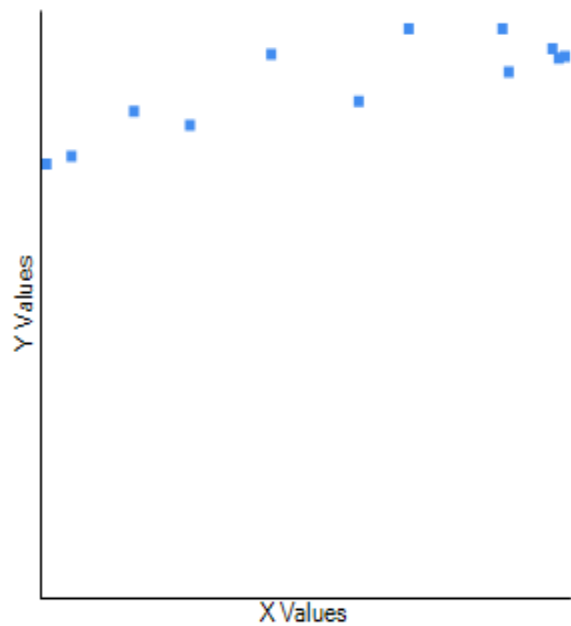
Fig. 5. Correlation between minimum and maximum temperature in Bandula.
