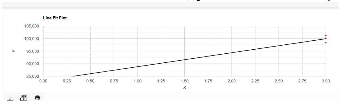
Figure 1. Air pressure correlated with latitudinal species richness in Antiphonus Attems, 1901.
