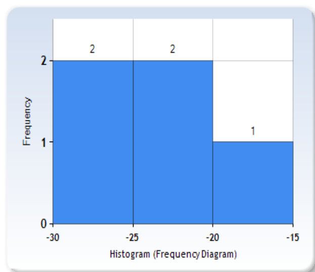
Figure 2. Latitudinal species richness in southern African Triaenostreptus Attems, 1914b.
