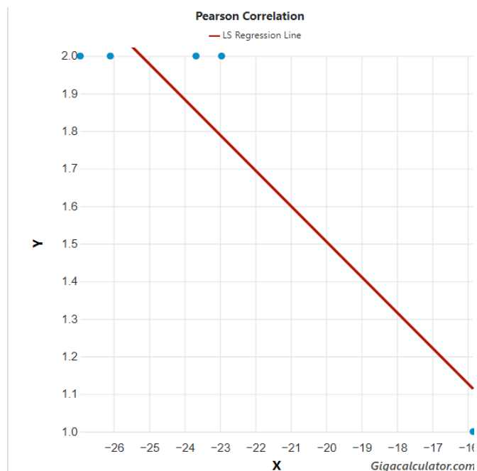
Figure 1. Latitude versus species richness in southern African Triaenostreptus Attems, 1914b.
