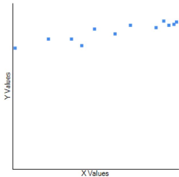
Fig. 2. Correlation between average and maximum temperature in Beira.
