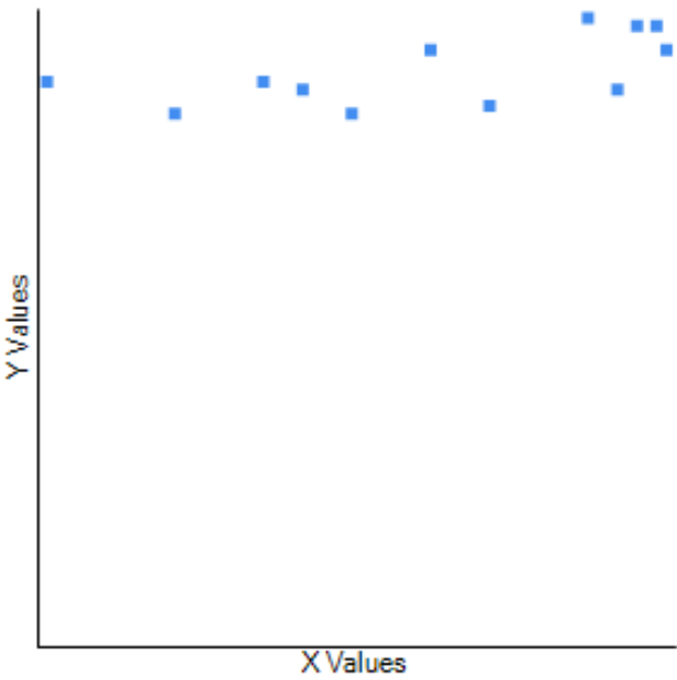
Fig. 4. Correlation between average temperature and humidity in Beira.
