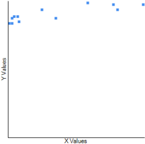
Fig. 9. Correlation between precipitation and humidity in Beira.
