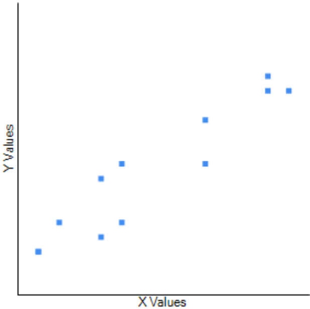
Fig. 11. Correlation between humidity and rainy days in Beira.
