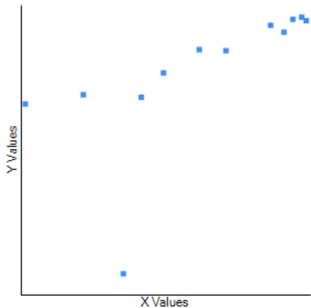
Fig. 1. Correlation between average temperature and minimum temperature in Beira.
