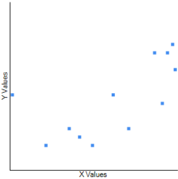
Fig. 5. Correlation between average temperature and rainy days in Beira.
