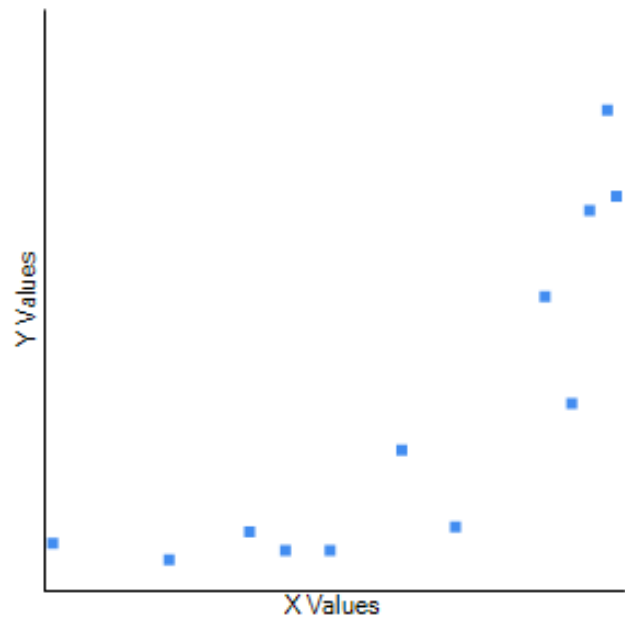
Fig. 3. Correlation between average temperature and precipitation in Beira.
