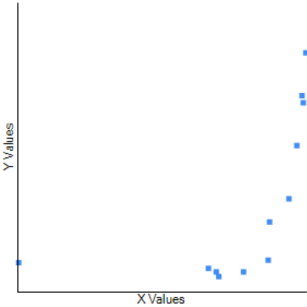
Fig. 7. Correlation between minimum temperature and precipitation in Beira.
