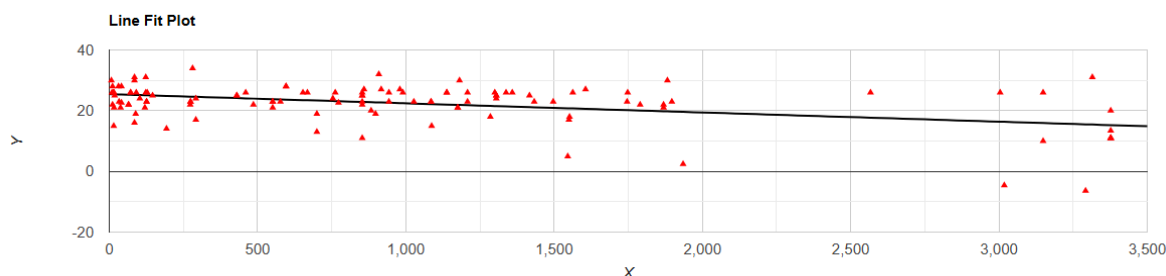
Figure 1. Temperature correlated to altitude in southern African Dalodesmidae Cook, 1896.
