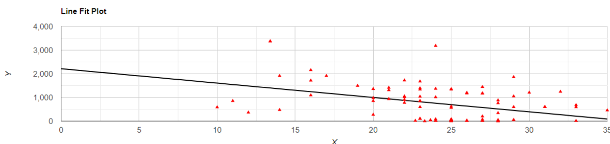
Figure 1. Correlation between temperature (x) and altitude (y) in Spinotarsus Attempts, 1909a.
