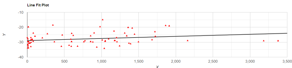
Figure 1. Correlation between latitude (y) and altitude (x) in southern African Spinotarsus Attempts, 1909a.
