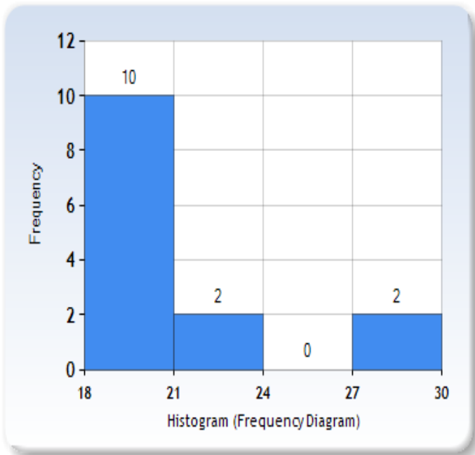
Figure 1. Longitudinal species richness in southern African Julomorpha Porat, 1872.
