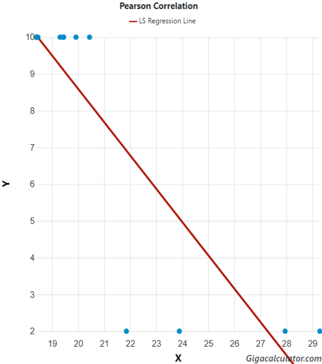
Figure 2. Longitude correlated with species richness in southern African Julomorpha Porat, 1872.
