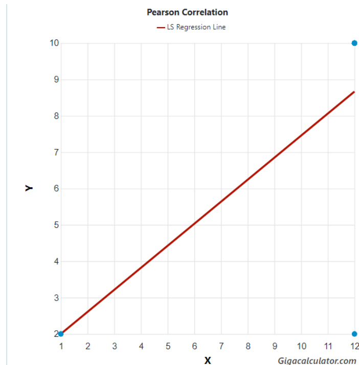
Figure 1. Longitudinal species richness correlated with latitudinal species richness in southern African Julomorpha Porat, 1872.
