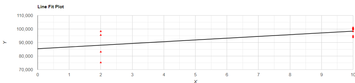
Figure 1. Longitudinal species richness correlated with air pressure in southern African Julomorpha Porat, 1872.
