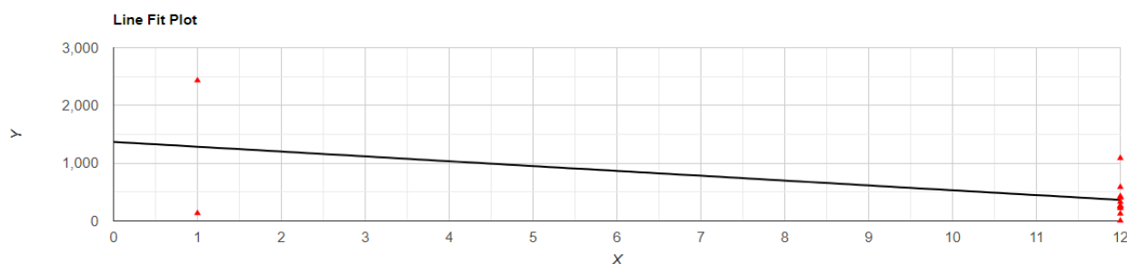
Figure 1. Latitudinal species richness correlated with altitude in southern African Julomorpha Porat, 1872.
