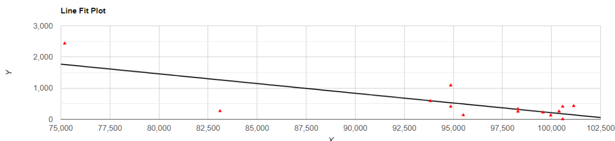
Figure 1. Air pressure correlated with altitude in southern African Julomorpha Porat, 1872.
