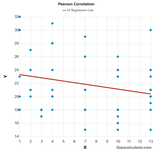
Figure 1. Latitudinal species richness correlated with temperature in Sphaerotheriidae Brandt, 1833.
