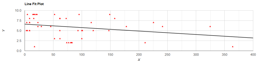
Figure 1. Distance to the nearest airport correlated with longitudinal species richness in Sphaerotheriidae Brandt, 1833.
