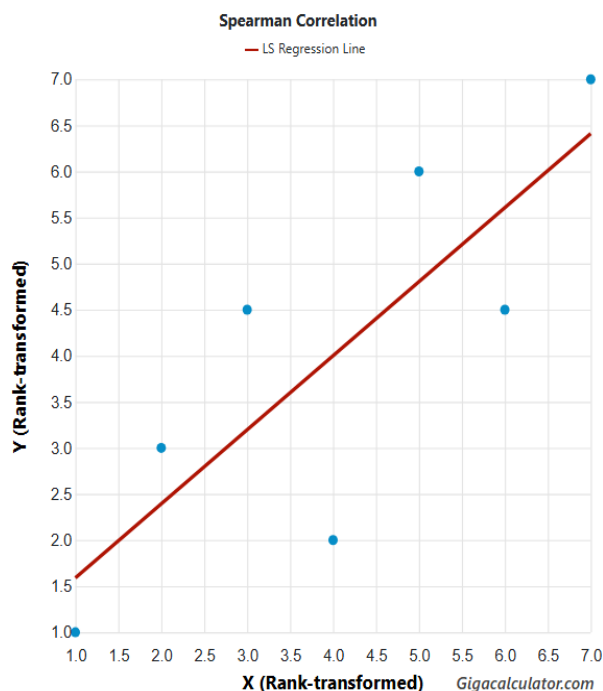
Figure 2. Minimum temperature correlated with body size in Sphaerotheriidae Brandt, 1833.
